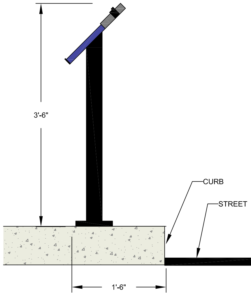
SIDE VIEW: MODIFIED SIGN - PREFERRED DESIGN
