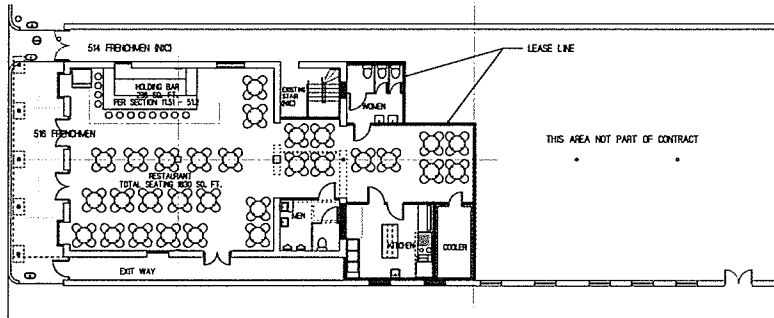
FURNITURE LAYOUT SCALE 1/8" = 1'-0"
