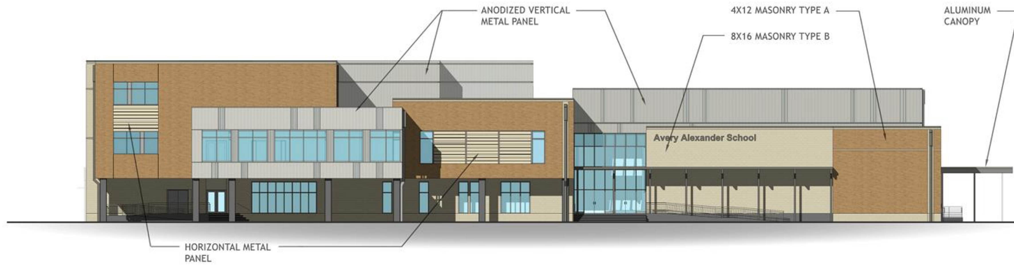
SAINT ROCH AVENUE ELEVATION
