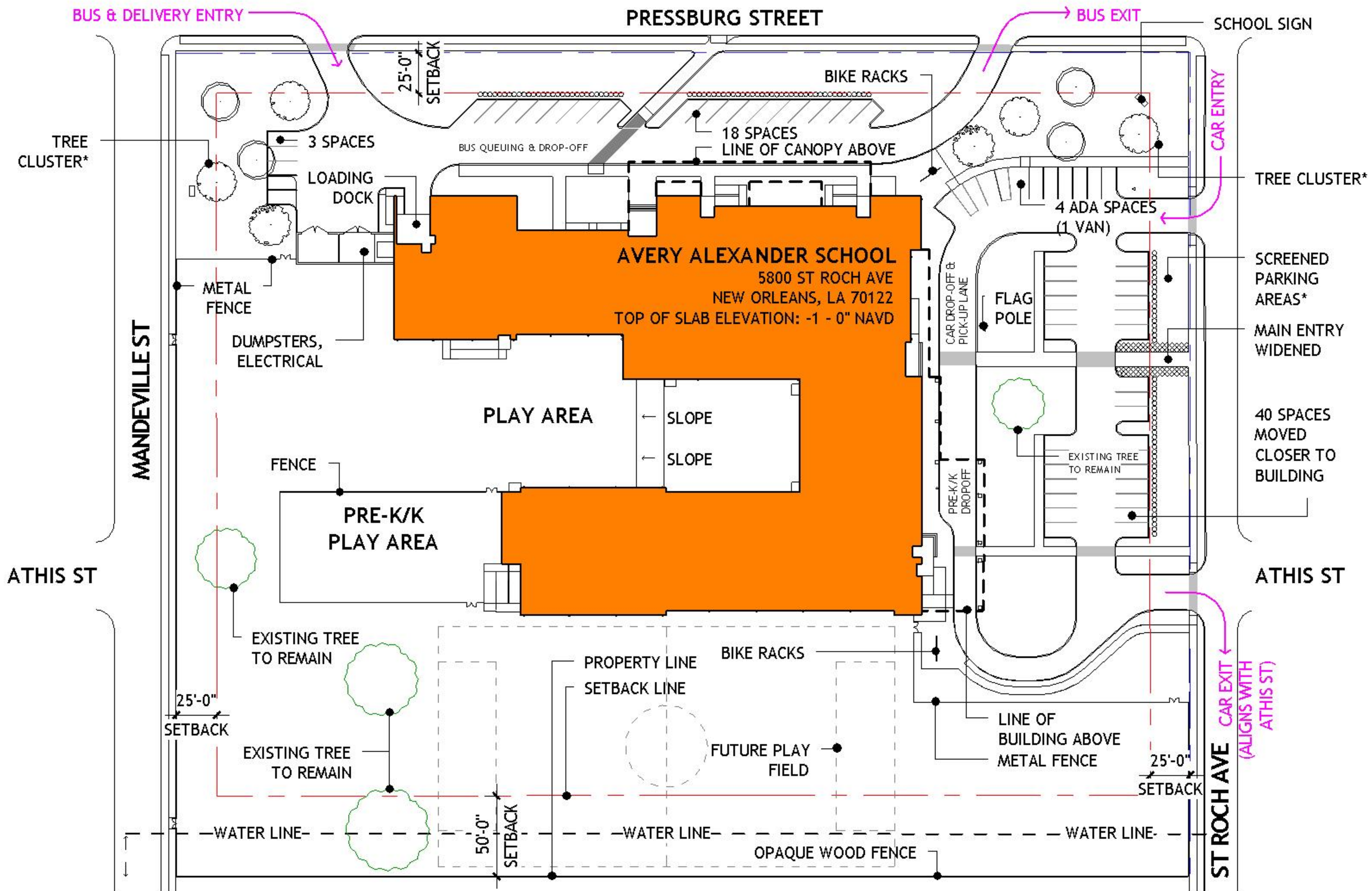
SITE PLAN
