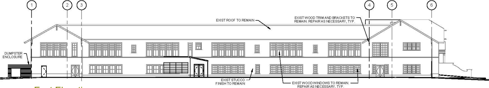
East Elevation
