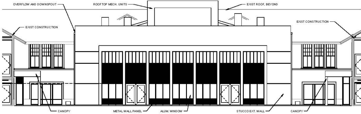
South Elevation Addition
