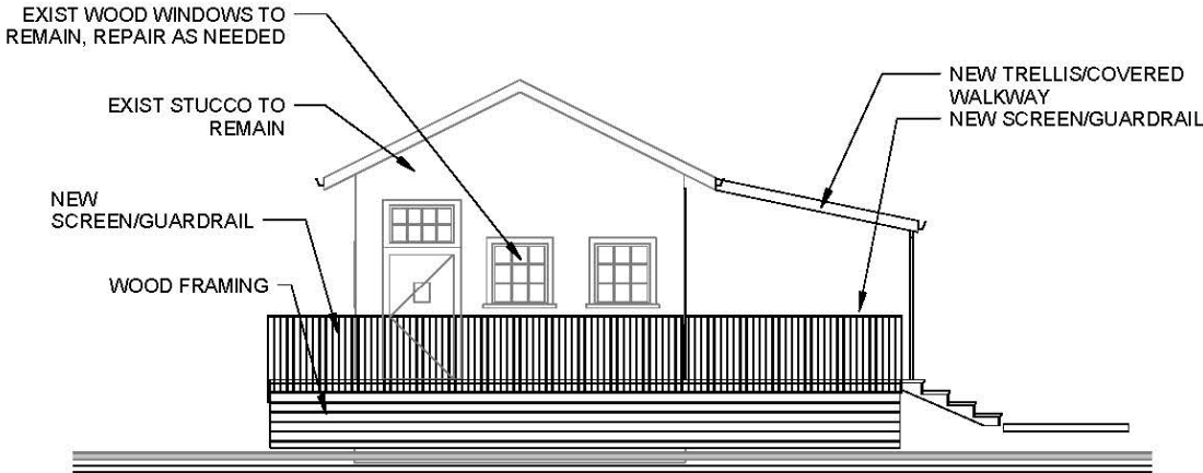
East Elevation
