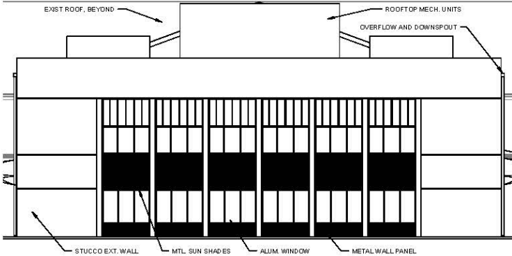
North Elevation Addition
