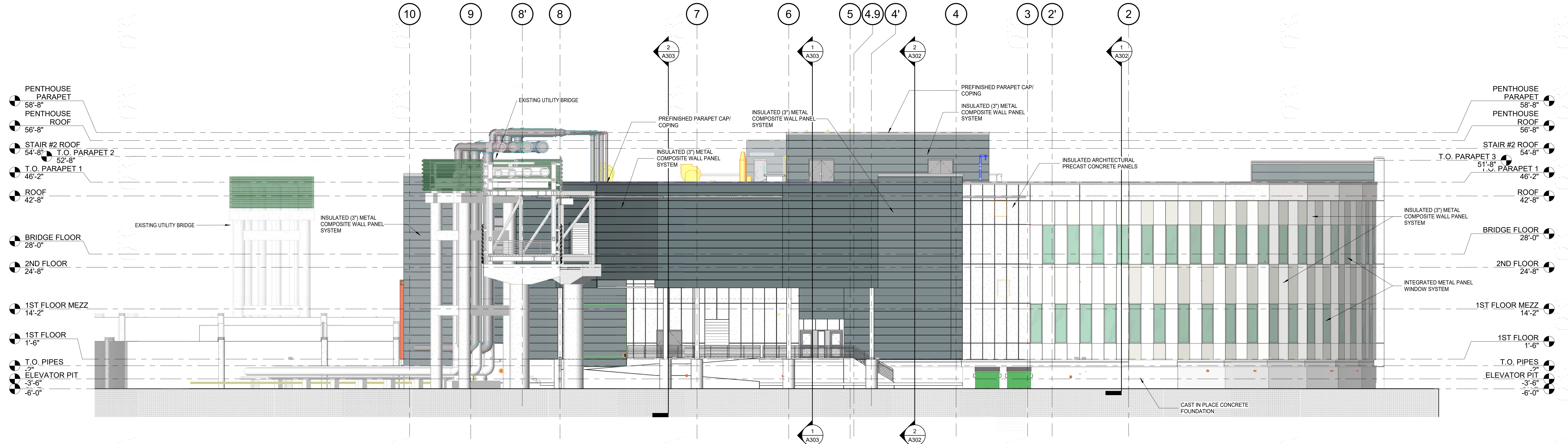
2 WEST ELEVATION 3/32" = 1'-0"
