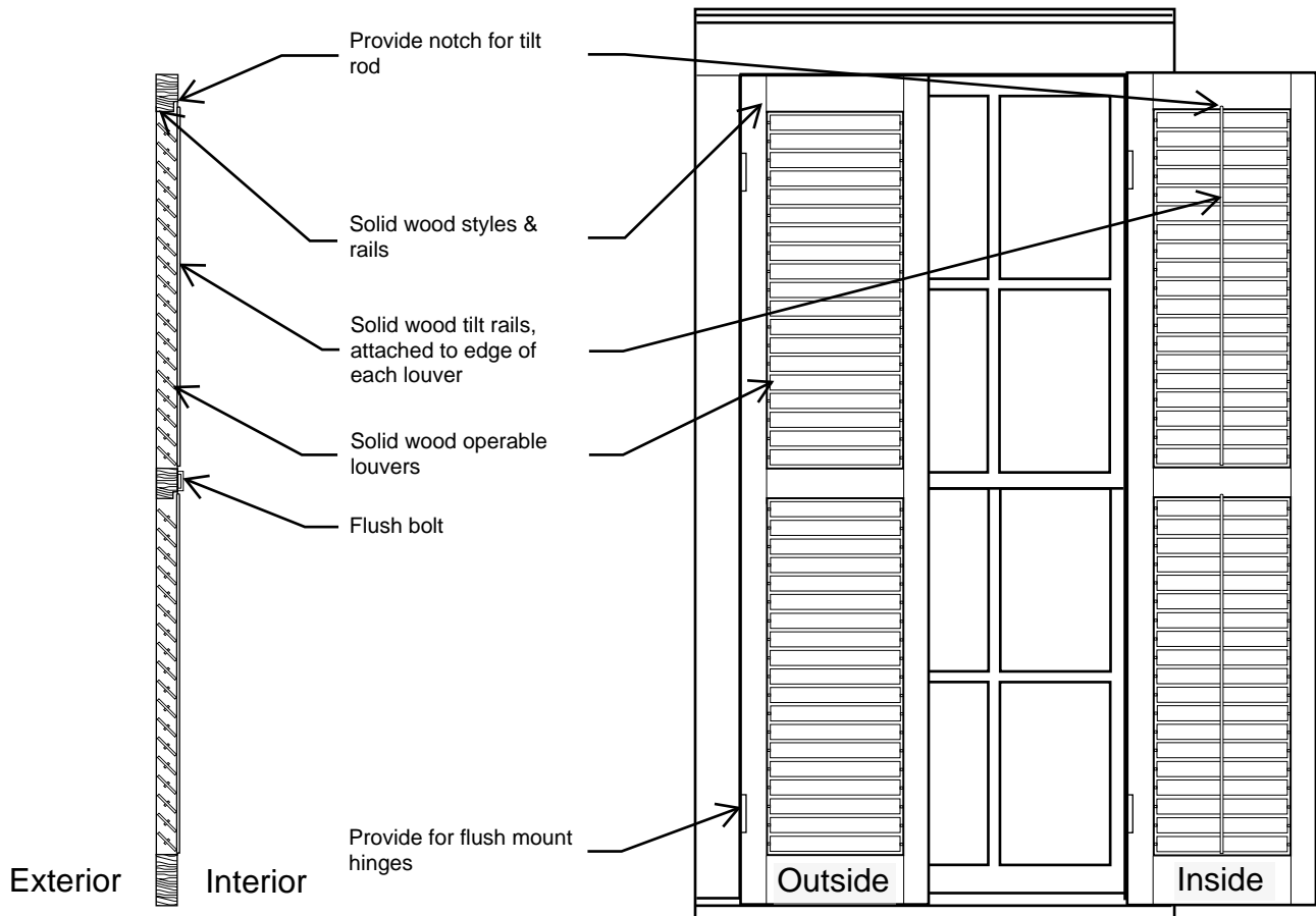
Vertical Section
