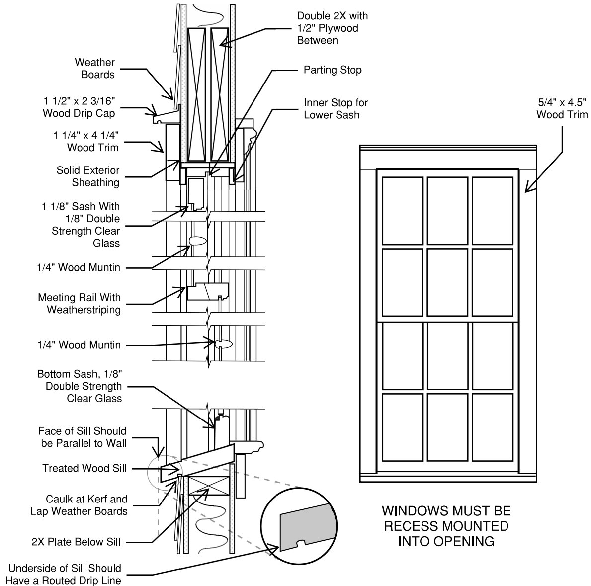
Section
