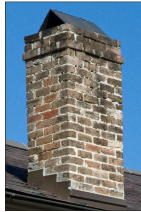
An inverted "V" cap is at the top of the chimney and flashing at its base.
