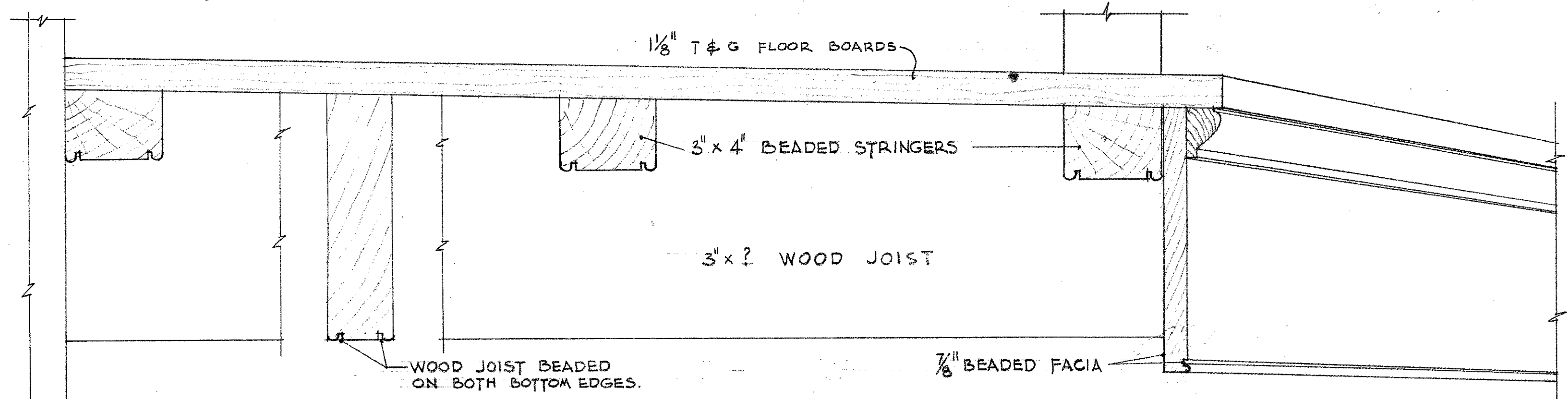
BALCONY DETAIL N° 2 SCALE 3" = 1'-0"
