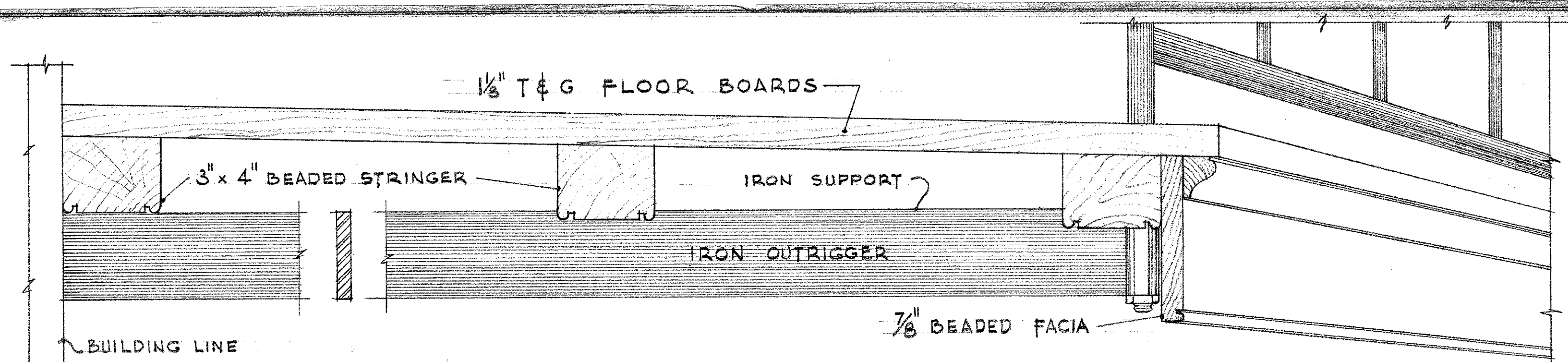
BALCONY DETAIL N° 1 SCALE 3" = 1'-0"
