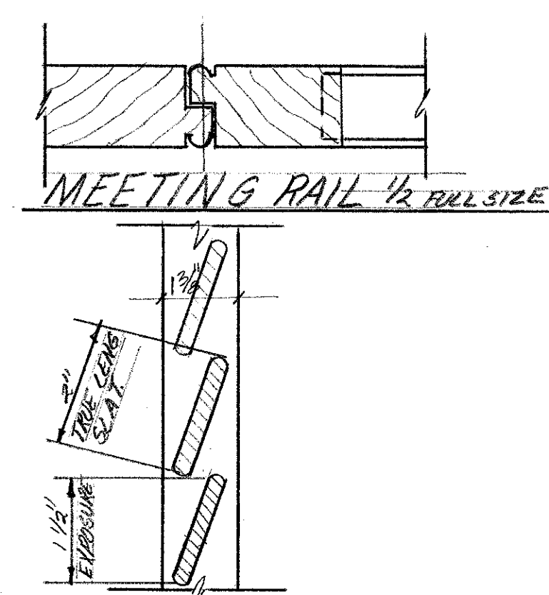
VERTICAL SECTION
