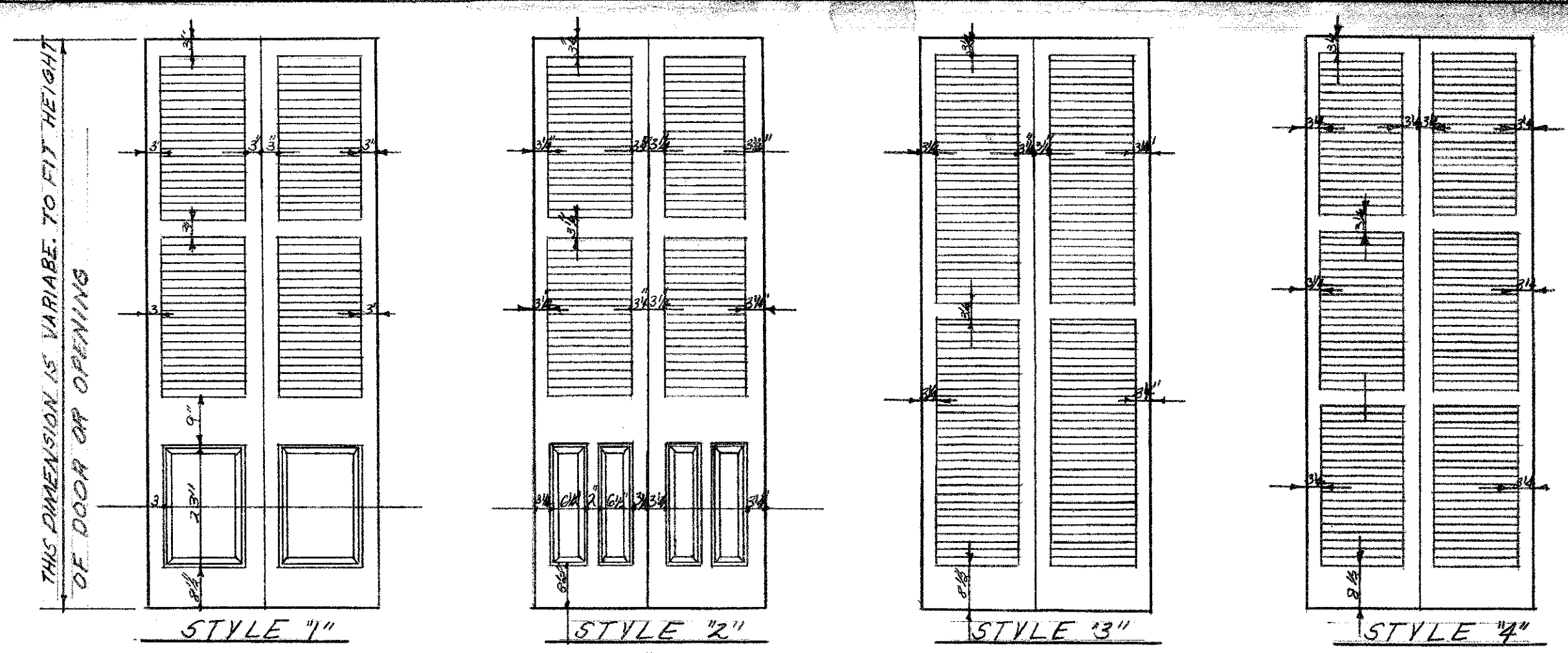
DOOR BLINDS + LOUVER & PANEL - SCALE: 1/2" = 1'-0"
