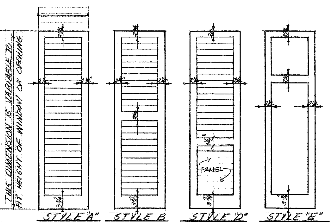
BLINDS + LOUVER & PANEL - SCALE: 3/4" = 1'-0" WINDOW BLINDS
