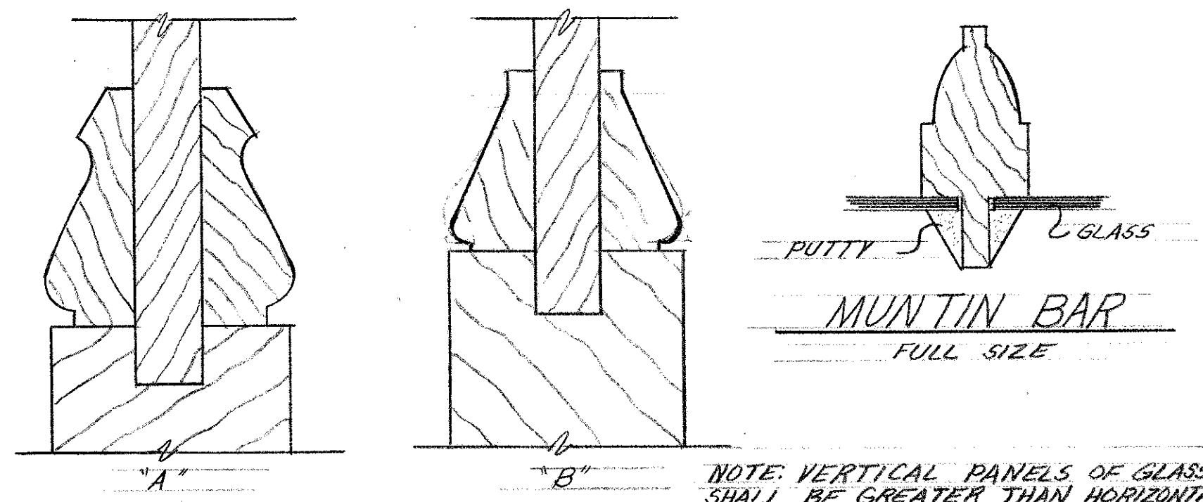
PANEL MOLDINGS FULL SIZE
