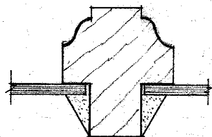
MUNTIN - I - F.S. PEYCHAUD HOUSE
