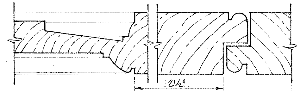
SECTION B-B FULL SCALE
