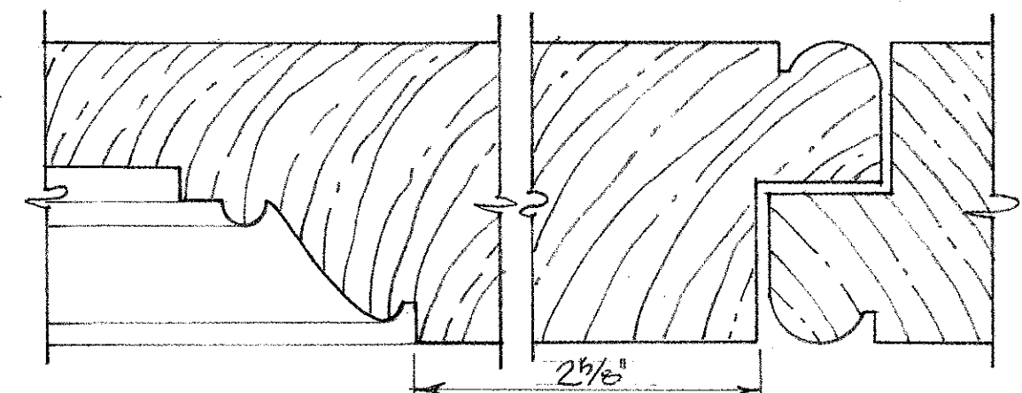
MEETING STILES OF BLINDS FULL SCALE
