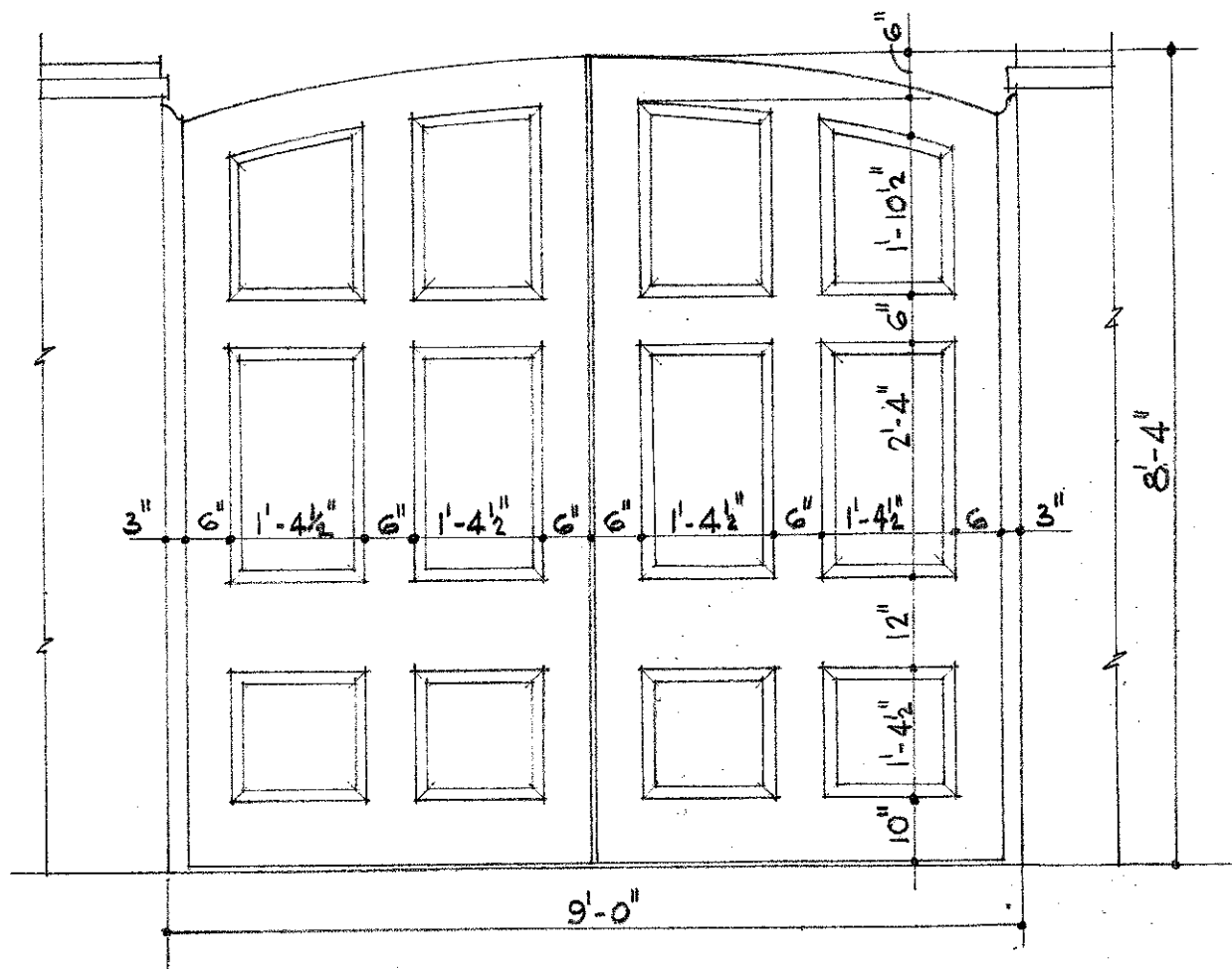
† GATE N o 1 † SCALE 1/2" = 1'-0"
