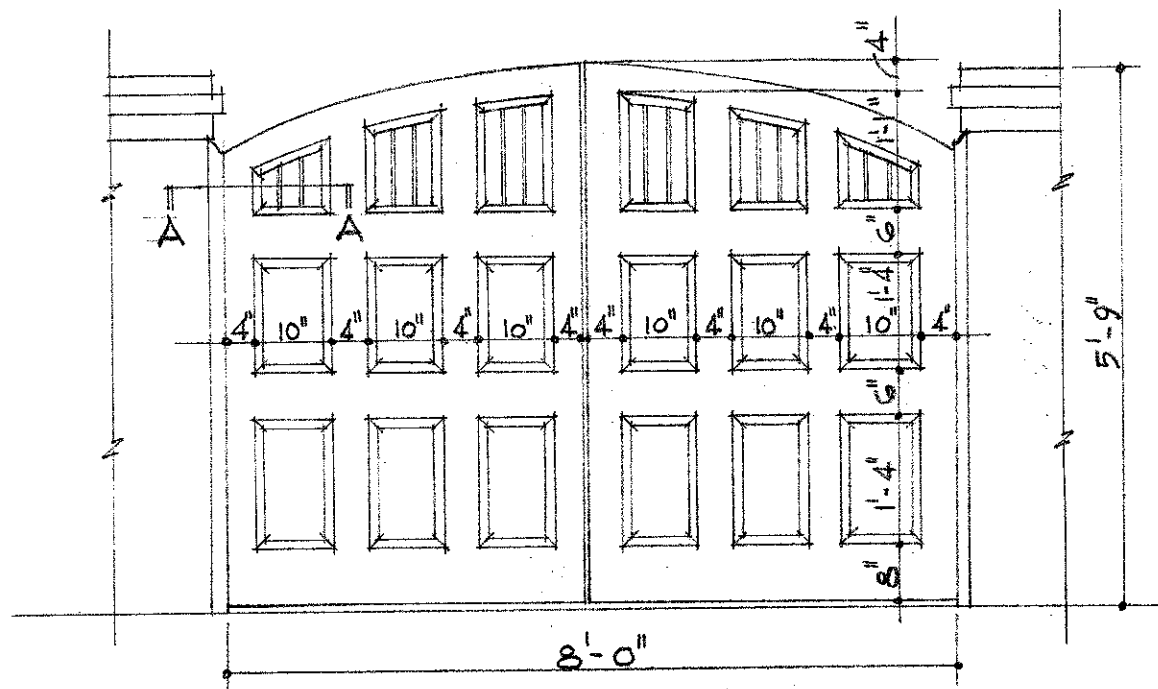
† GATE N o 3 † SCALE 1/2" = 1'-0"
