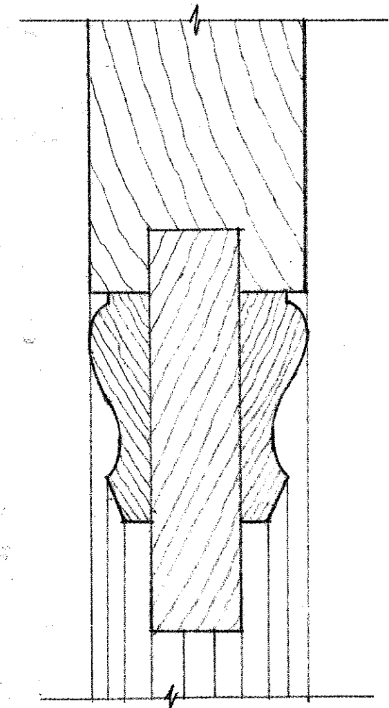
† TYPICAL DETAIL † FULL SIZE USE THIS MOULDING FOR ALL PANELS.
