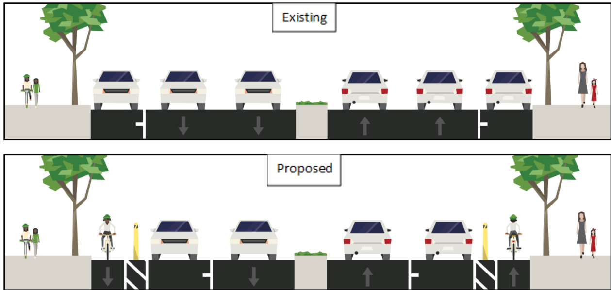
Existing and proposed typical roadway cross sections for Bienville Avenue (N. Norman C Francis Parkway to N. Carrollton Avenue)
