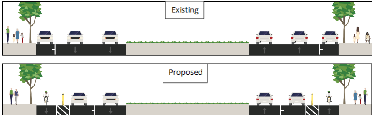
Existing and proposed typical roadway cross sections for Franklin Avenue (St. Claude Avenue to N. Dorgenois Street)
