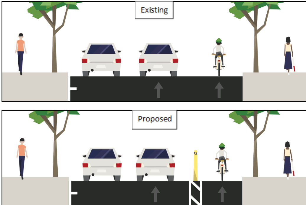
Existing and proposed typical roadway cross sections for North Galvez Street (Orleans Avenue to Franklin Avenue)
