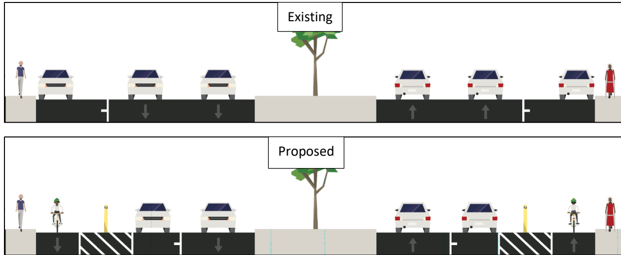
Existing and proposed roadway cross sections for South Galvez Street (Martin Luther King Jr Blvd to Erato Street)
